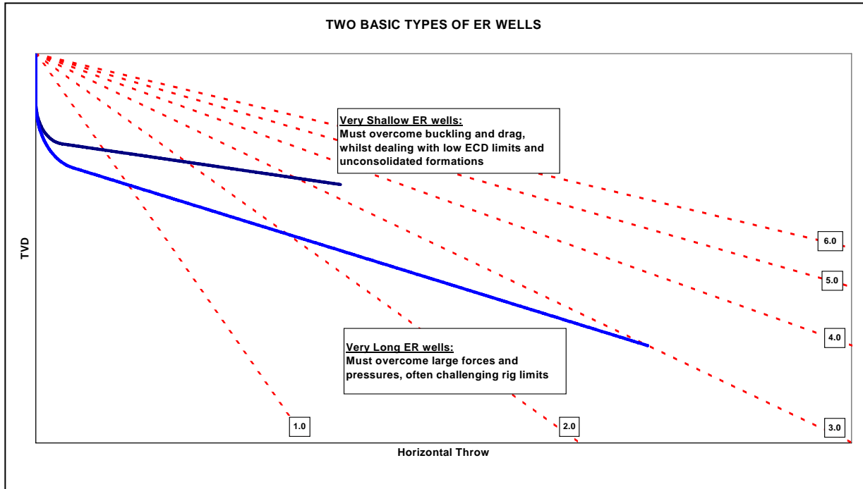
Characteristics of Very Shallow and Very Long ERD Wells
