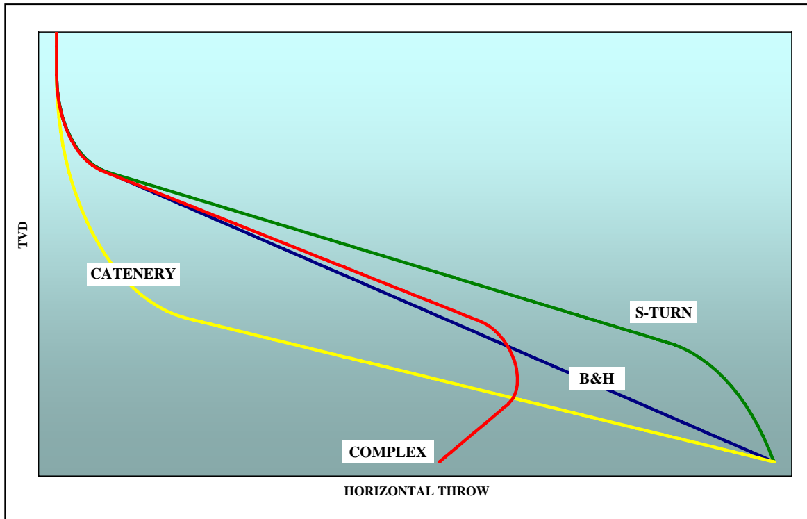
Well Profile Options for ERD Wells
